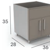
SINK BASE Width: 36" (SB36)
